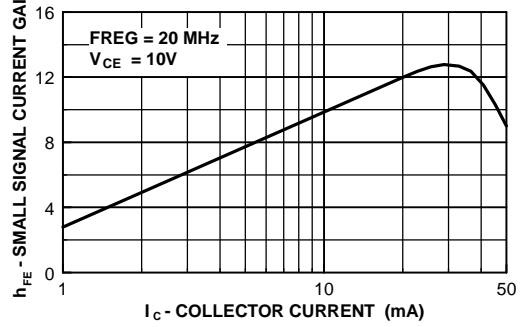
Small Signal Current Gain vs Collector Current
