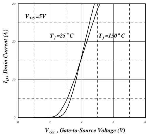
Fig 11. Transfer Characteristics
