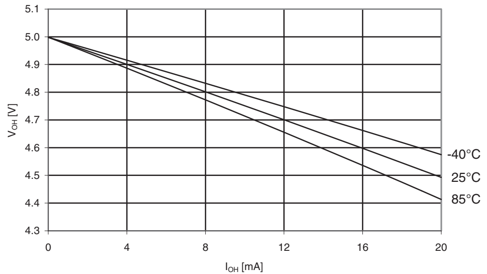
Figure 29-24. Atmel ATmega164A: I/O pin output voltage vs. source current ( V_{CC} = 5V ).
