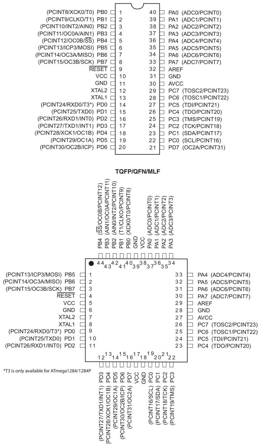
Figure 1-1. Pinout.
