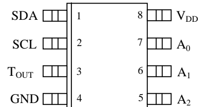
DS1621S 8-PIN SO (150mil) DS1621V 8-PIN SO (208mil) See Mech Drawings Section
