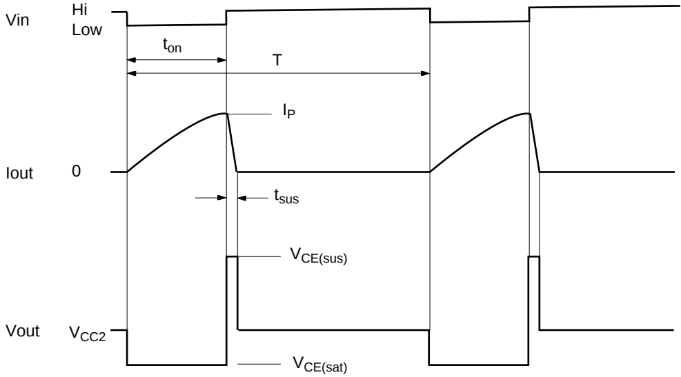
Figure 1 Output Waveforms
