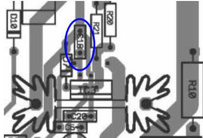
Figure 2 Detail X, Soft Start Capacitor C18 Layout Recommendation
