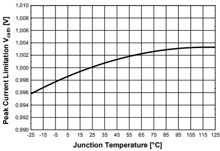
Figure 48 Peak Current Limitation V_{csth} vs. T_j
