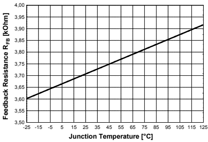
Figure 42 Feedback Resistance R_{FB} vs. T_j
