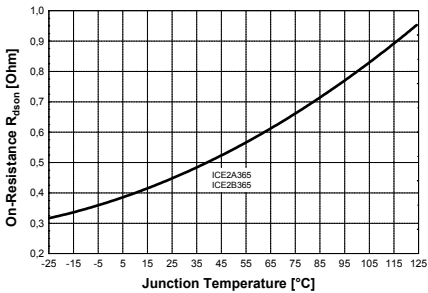
Figure 50 Drain Source On-Resistance R_{DSon} vs. T_j
