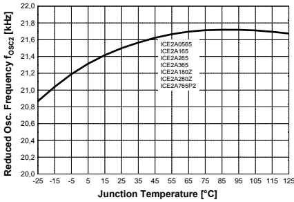
Figure 36 Reduced Osc. Frequency f_{OSC2} vs. T_j
