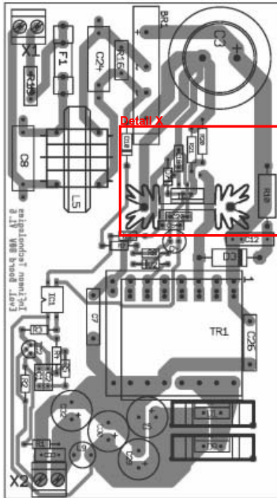
Figure 1 Layout of Board EVALSF2_ICE2B765P2
