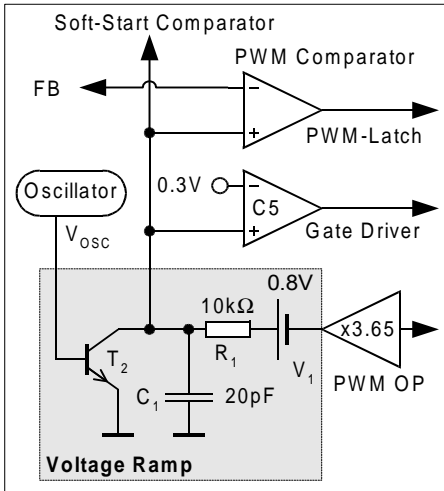
Figure 8 Improved Current Mode
