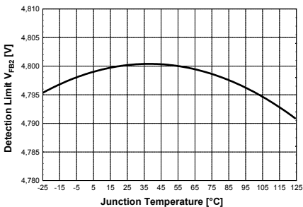
Figure 44 Detection Limit V_{FB2} vs. T_j
