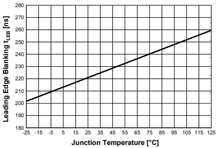
Figure 49 Leading Edge Blanking V_{VCC1} vs. T_j
