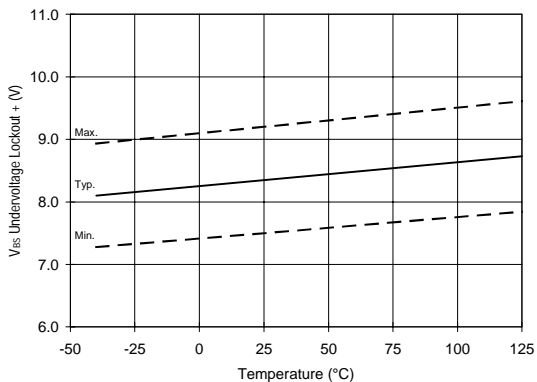
Figure 33. V_{BS} Undervoltage (+) vs. Temperature
