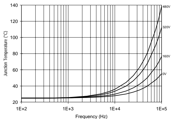
Figure 54. IR2130/IR2132 T J vs. Frequency (IRF450) R GATE = 10Ω, V CC = 15V
