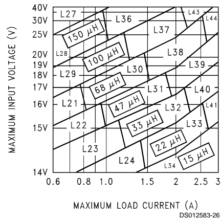
FIGURE 6. LM2596-12
