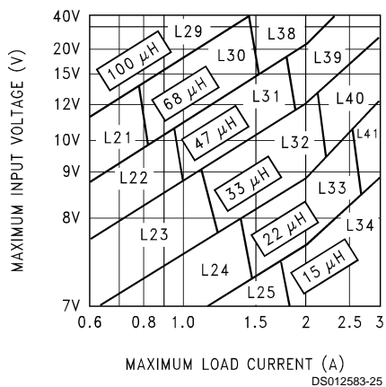
FIGURE 5. LM2596-5.0
