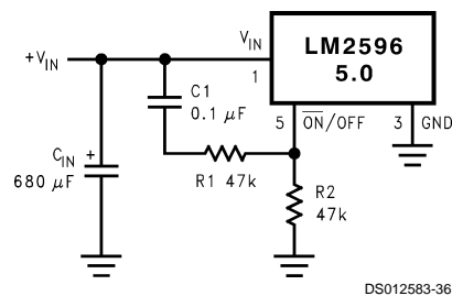
FIGURE 21. Delayed Startup
