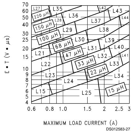
FIGURE 7. LM2596-ADJ
