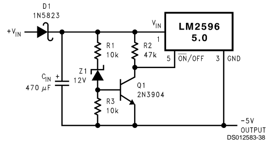
FIGURE 23. Undervoltage Lockout for Inverting Regulator
