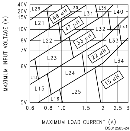
FIGURE 4. LM2596-3.3
