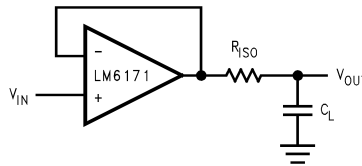
Figure 61. Isolation Resistor Used to Drive Capacitive Load
