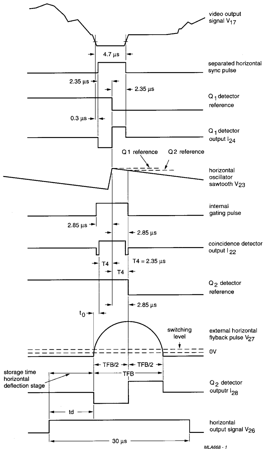
Fig.9 Timing diagram.
